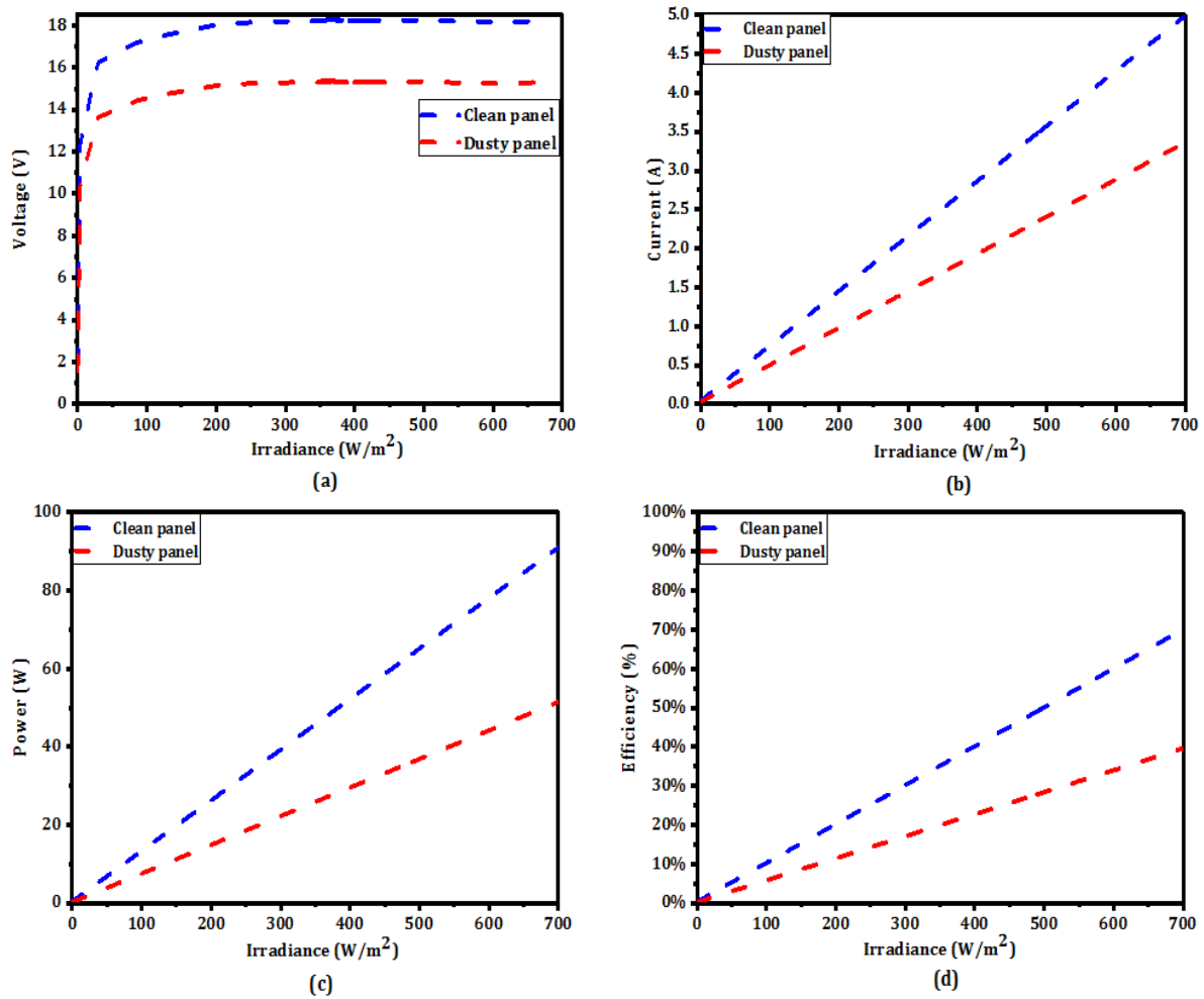
Fig. 8. impact of irradiance on operating voltage, current, power and efficiency for clean and clean and dusty panels
