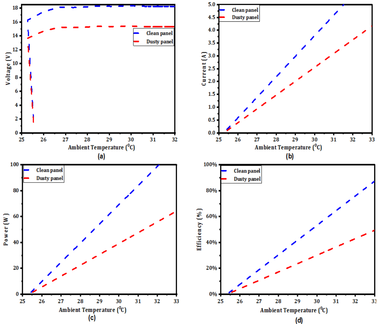
Fig. 6. impact of ambient temperature on operating voltage, current, power and efficiency for clean and clean and dusty panels
