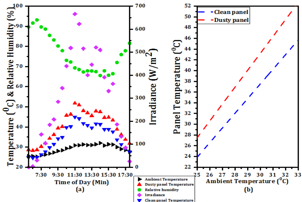
Fig. 5. Climatic condition at site and panel temperatures with respect to ambient temperature
