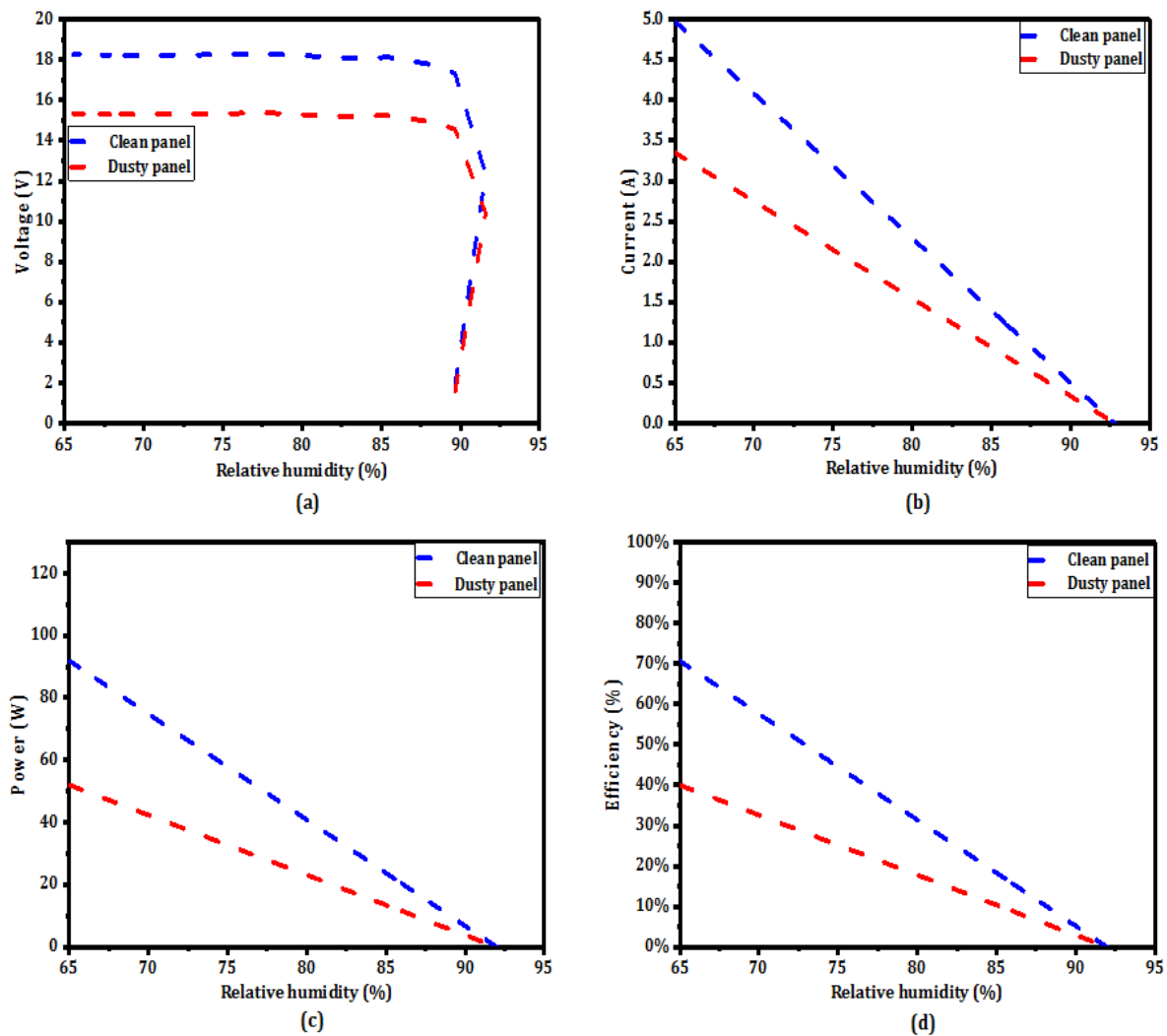
Fig. 7. impact of relative humidity on operating voltage, current, power and efficiency for clean and clean and dusty panels
