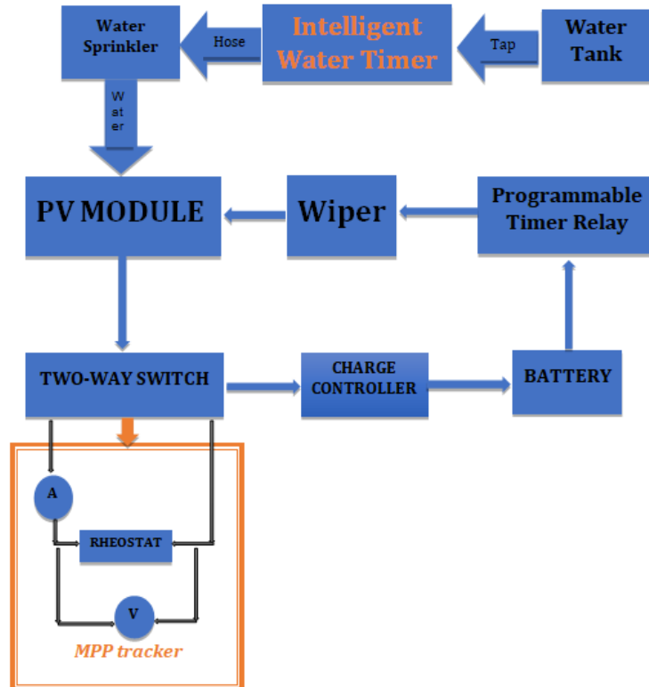
Fig. 3. The experimental setup for the clean panel
