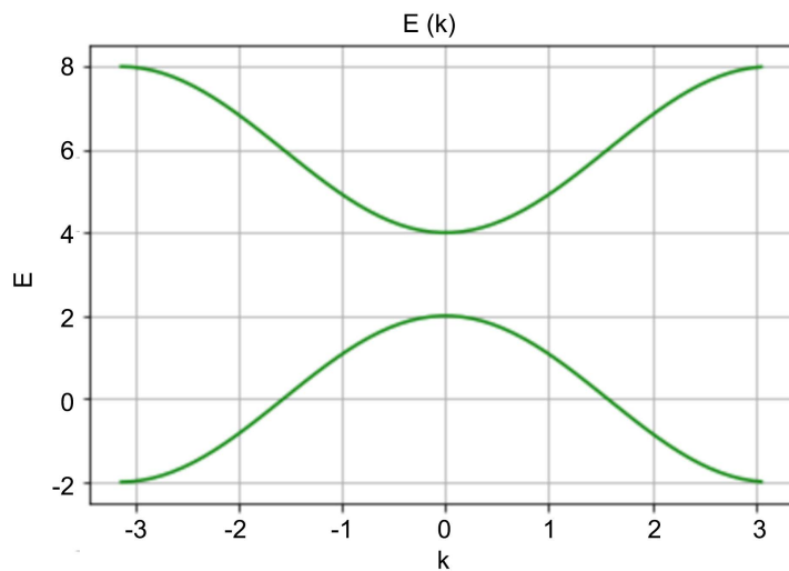
Figure 1. The standard energy dispersion relation in solids with energy gap separating conducting and valence band.
