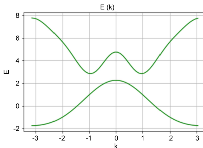
Figure 3. Energy dispersion curves with minimal energy of conducting band in different value of lattice momentum comparing with maximum energy of valence band.
