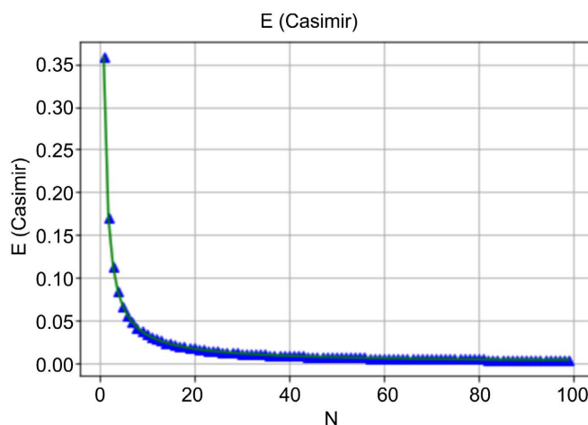
Figure 4. Casimir energy graph for 1 + 1 dimensional lattice for different numbers of lattice nodes.
