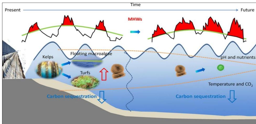
Fig. 3. Comparative effects of normal and heatwave conditions in oceans (Source: IITM, Pune)
