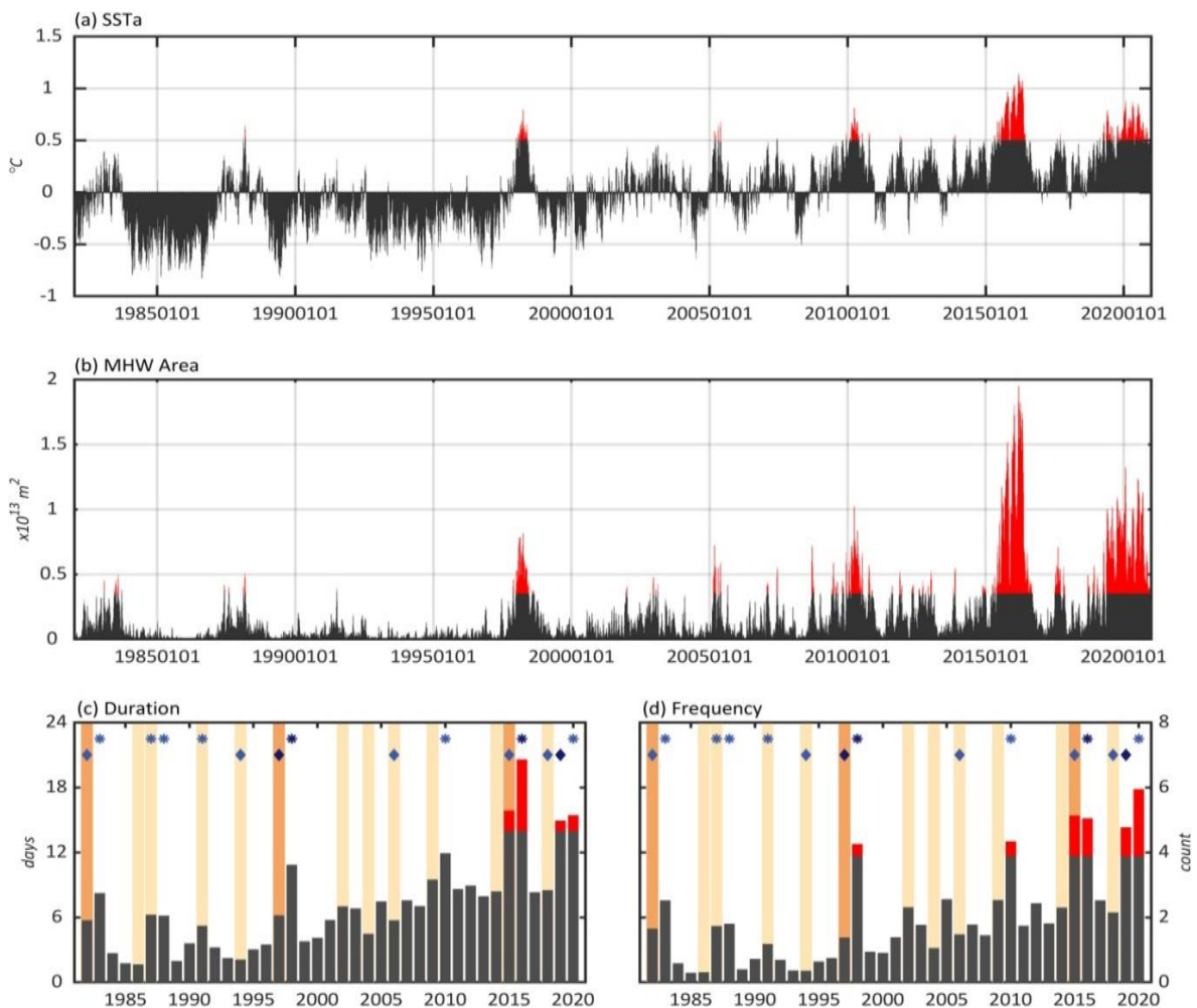
Fig. 1. Long-Lasting Marine Heatwaves Instigated by Ocean Planetary Waves in the Tropical Indian Ocean during 2015–2016 and 2019–2020
