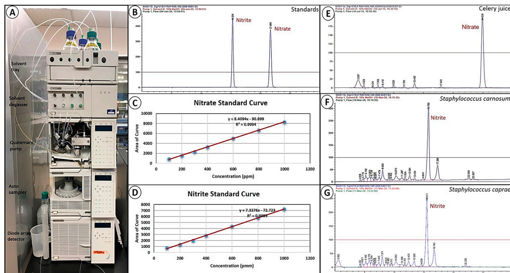
Figure 4. Analysis of nitrate and nitrite using C_8 -RP ion-pairing high performance liquid chromatography (HPLC). Panel (A): HPLC system. Panel (B): chromatogram of nitrite and nitrate standards. Panel (C): standard curve of nitrate standards. Panel (D): standard curve of nitrite standards. Panel (E): celery juice extract. Panel (F): celery juice extract fermented with industry standard strain, Staphylococcus carnosus . Panel (G) celery juice extract fermented with bacterial isolate, Staphylococcus caprae .
