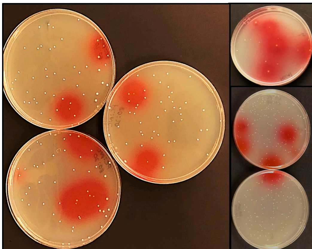
Figure 3. Nitrate reducing bacterial colonies showing red color zones after sandwich overlays with soft agar containing nitrate reagents A and B. Colonies with surrounding red color were isolated using the inverted agar method and streak plated on new plates and confirmed for nitrate reduction in nitrate broth (the plates above are shown from the bottom side of the petri plate).
