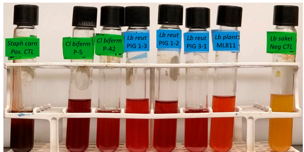
Figure 2. Nitrate reduction test performed on M17-nitrate broth culture broths of various strains from culture collections including: Staphylococcus carnosus (positive control), Clostridium bifermentans P-5, Clostridium bifermentans P-42, Lactobacillus reuterii PIG 1-3, Lactobacillus reuterii PIG 1-2, Lactobacillus reuterii PIG 3-1, Lactobacillus plantarum ML811, and Lactobacillus sakei (negative control). The red color generated after addition of sulfanilic acid and alpha-naphthylamine signifies the presence of nitrite (reduced from nitrate). The bacterial identities were determined by 16S rRNA sequence analysis.
