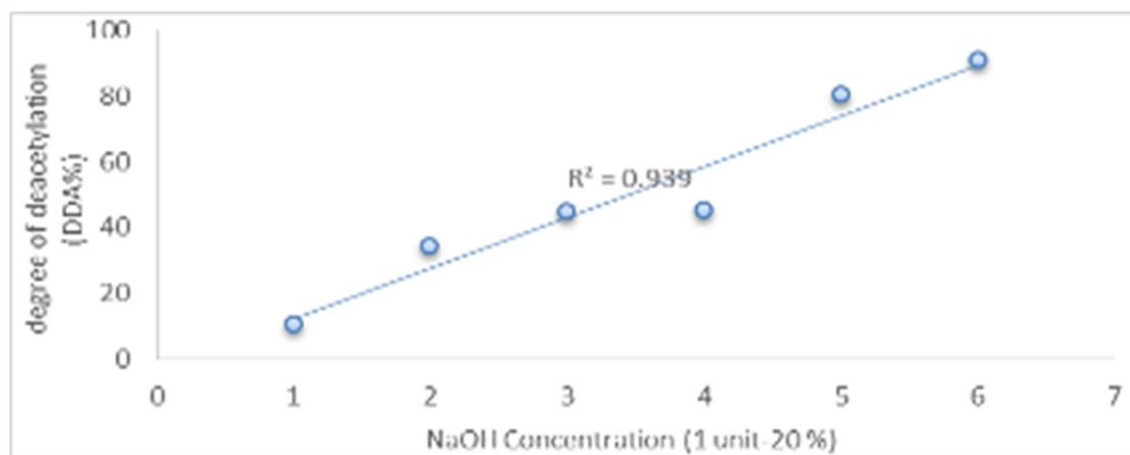
Fig. 4. Linear fit for deacetylation of chitin using sodium hydroxide
