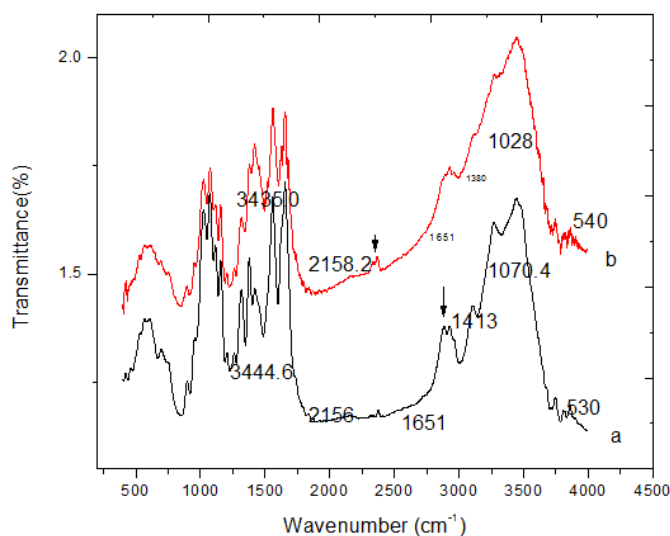
Fig. 5. FTIR spectra of a) chitin and b) chitosan
