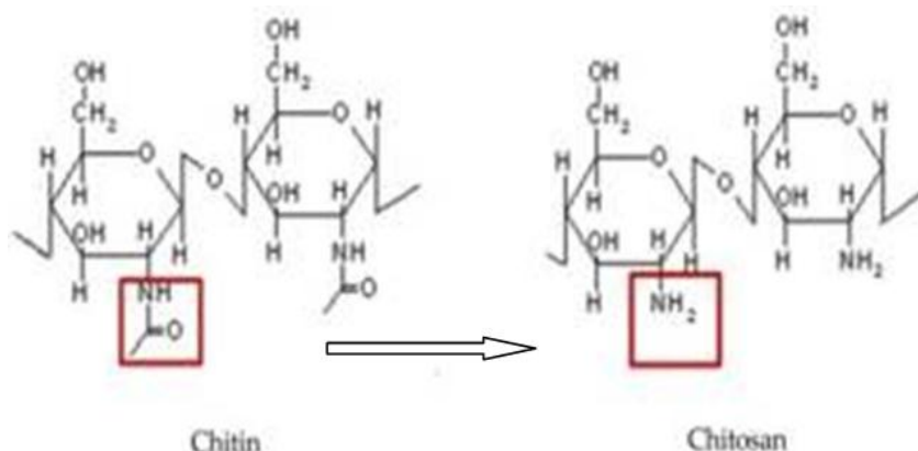
Fig. 1. Structural formula of chitin and chitosan [20]
