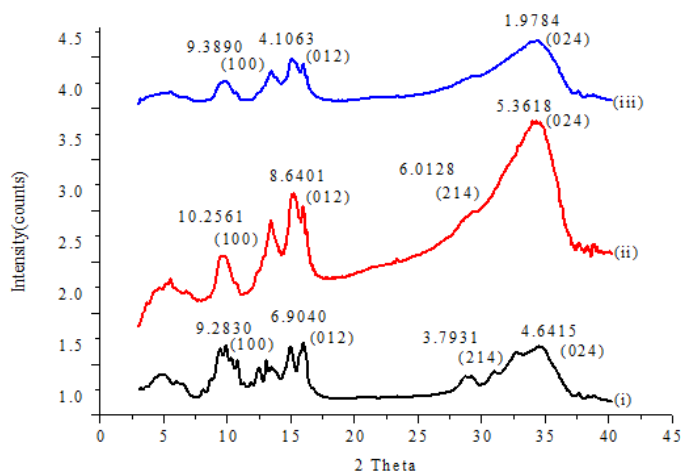
Fig. 7. X-Ray Diffractograms of; (i) Chitin, (ii) Chitosan nanoparticle and (iii) CISNC
