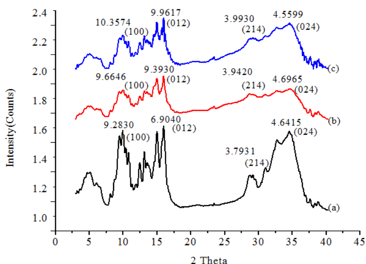
Fig. 6. XRD diffractograms for (a) Chitin, (b) Chitosan and (c) Chitosan-nanoparticle
