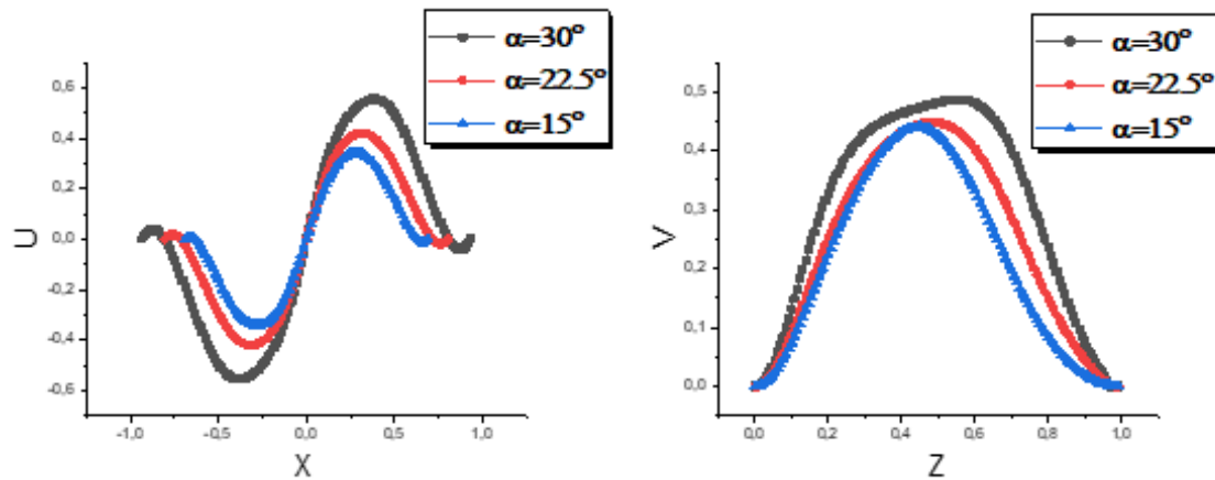
Fig. 9. Longitudinal and transverse velocity profiles for various wall slopes
