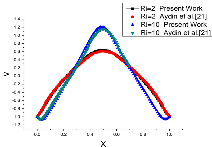
Fig. 3. Comparison of the nondimensional vertical velocity profiles at the vertical midplane of the cavity for Ri=2 and for Ri=10 (results of Aydin et al. [21] and present work)
