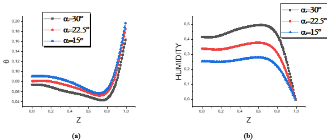
Fig. 10. Longitudinal temperature (a) and moisture (b) profiles for various wall slopes
