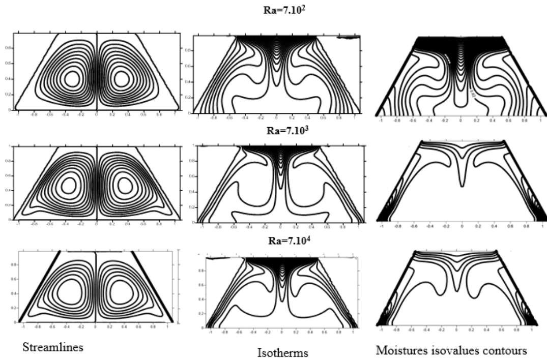
Fig. 13. Effect of Rayleigh number on streamlines, isotherms and moisture isovalues
