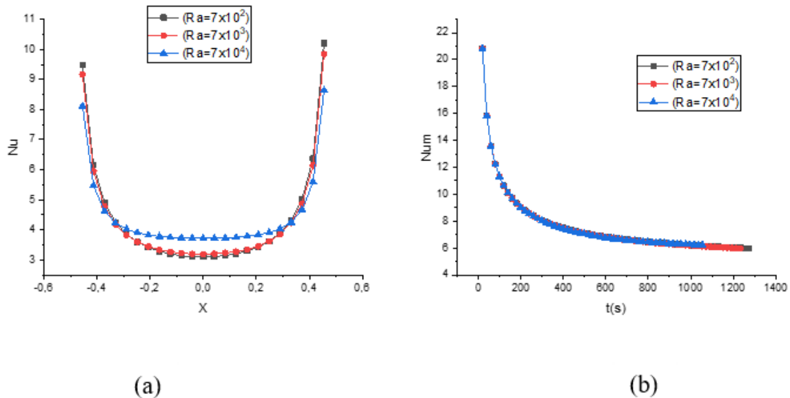
Fig. 18. Effect of the Rayleigh number on the local Nusselt and average Nusselt number
