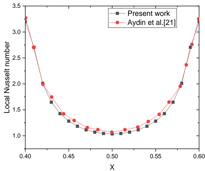
Fig. 4. Comparison of local Nusselt number of the present work and that of Aydin et al. [21] for Ri=10
