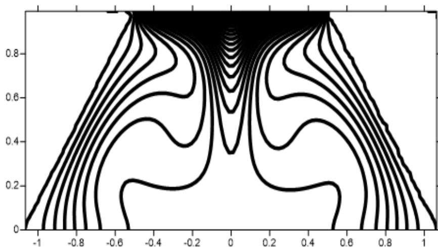
Fig. 6. Distribution of isothermal lines for Pr=0.71 ; F=1 ; Ra=7.10^2
