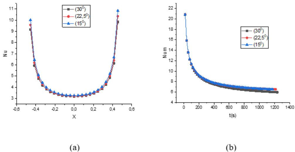
Fig. 17. Effect of walls inclination angle on the local Nusselt (a) and average Nusselt number (b)
