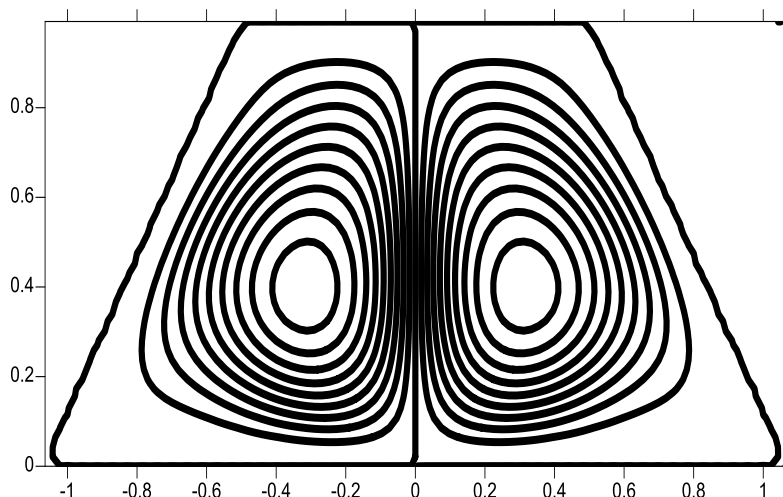
Fig. 5. Distribution of streamlines for Pr=0.71 ; F=1 ; Ra=7.10^2
