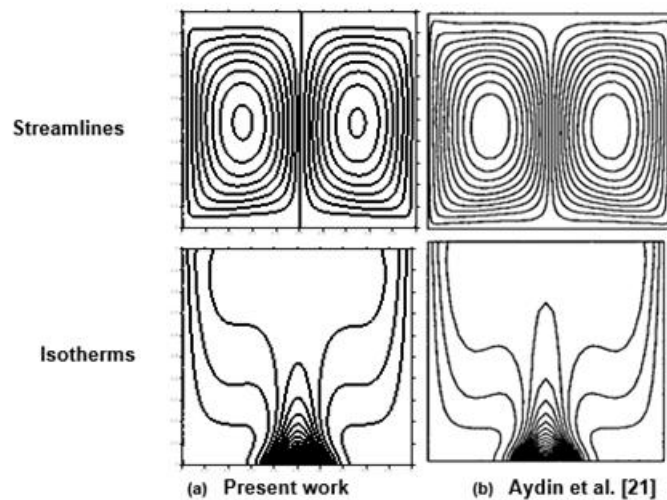
Fig. 2. Comparison of streamlines lines and isotherms of the present work (a) with that of Aydin et al. [21]
