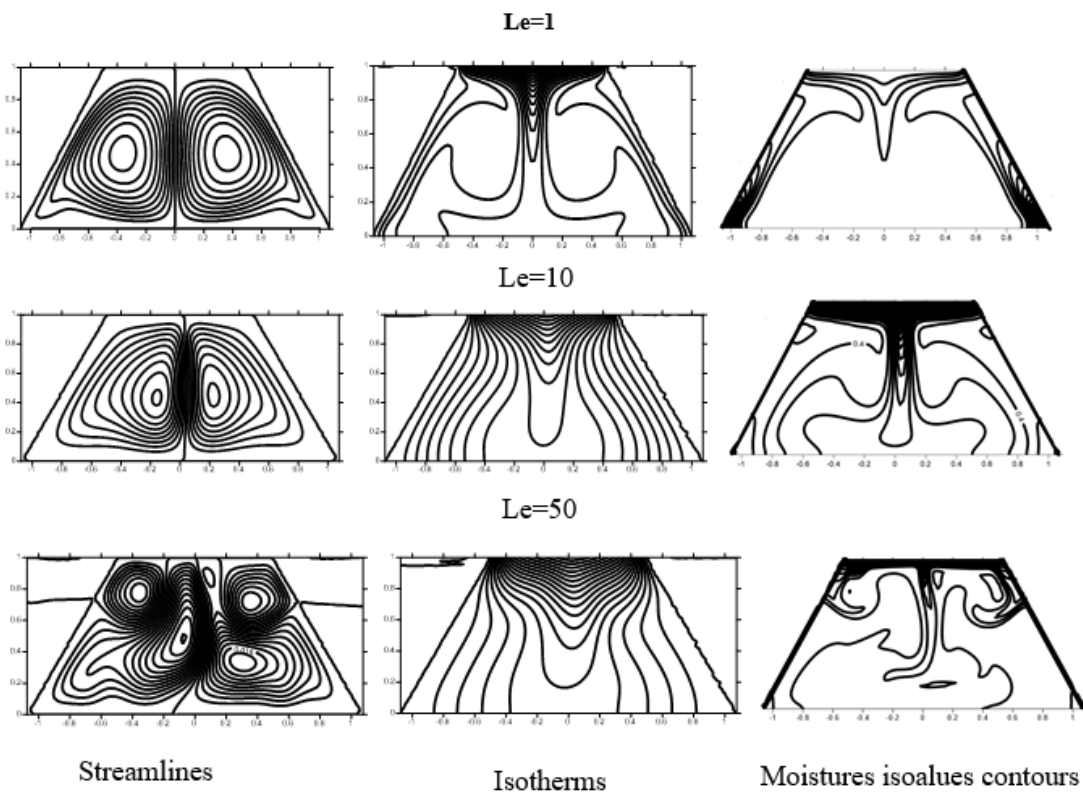
Fig. 15. Effect of Lewis number on the Stream lines, Isotherms and Moisture isoalues
