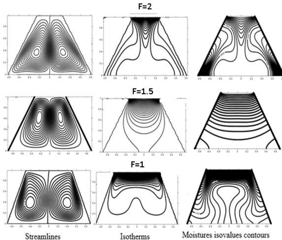
Fig. 11. Influence of the geometrical form factor on streamlines, isotherms and isovals of humidity
