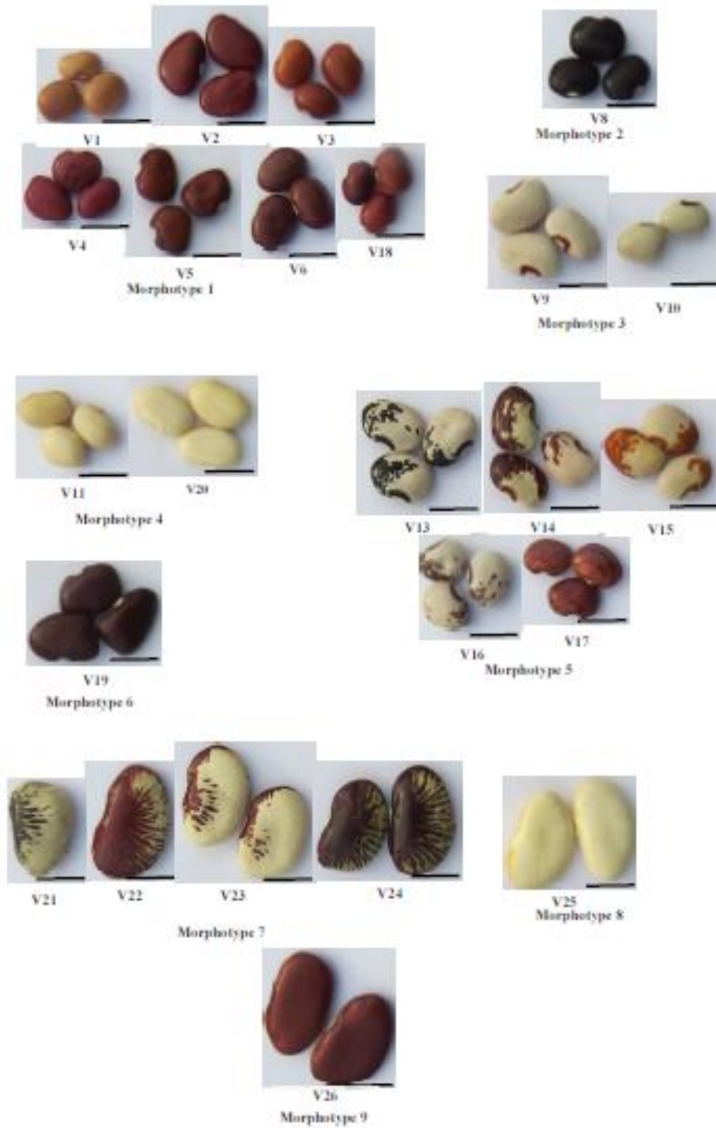
Fig. 2. Morphotypes of Phaseolus lunatus grown in Benin
