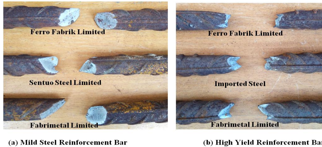
Fig. 9. Typical Reinforcement Bars in Ghana at Failure
