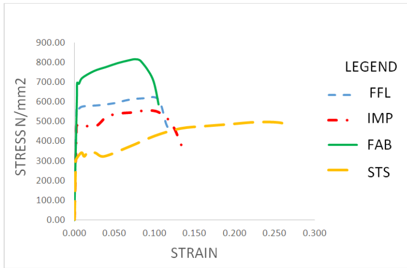
Fig. 6. Stress-Strain plot of 16mm nominal diameter high yield reinforcing bars
