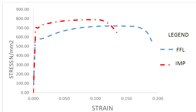
Fig. 8. Stress-Strain plot of 25mm nominal diameter high yield reinforcing bars
