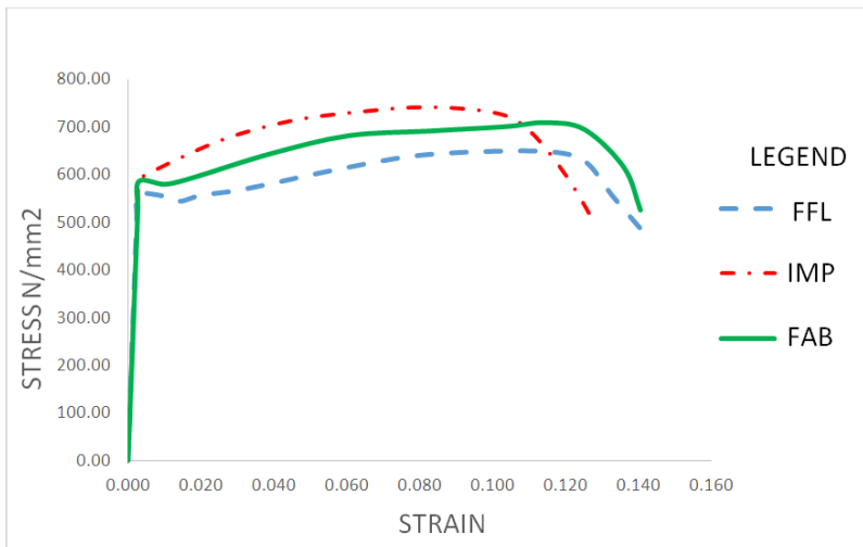
Fig. 7. Stress-Strain plot of 20mm nominal diameter high yield reinforcing bars
