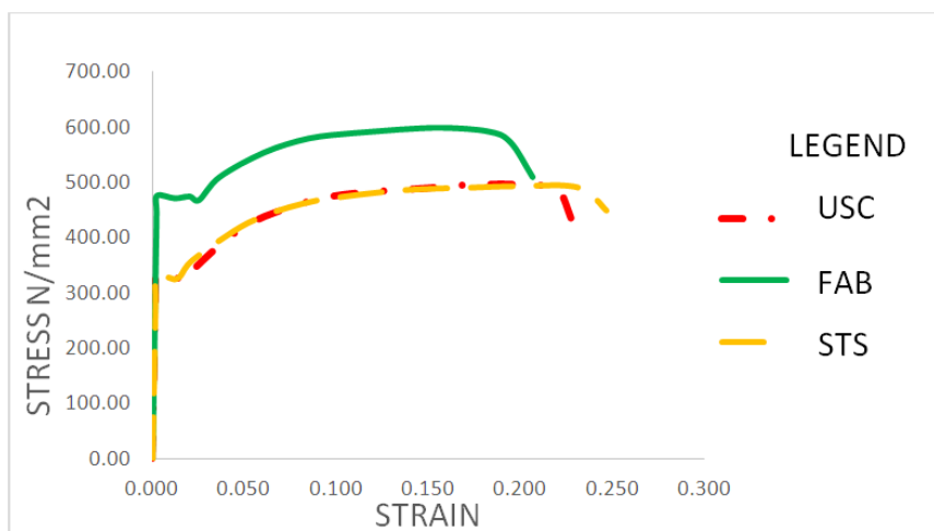
Fig. 4. Stress-Strain plot of 20mm nominal diameter mild steel ribbed reinforcing bars
