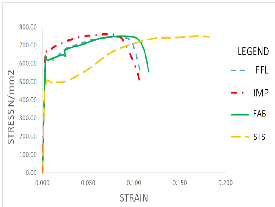
Fig. 5. Stress-Strain plot of 12mm nominal diameter high yield reinforcing bars
