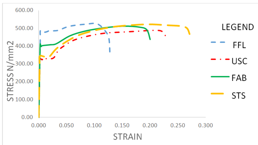
Fig. 3. Stress-strain plot of 16mm nominal diameter mild steel ribbed reinforcing bars
