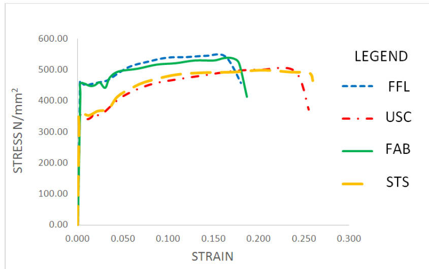
Fig. 2. Stress-Strain plot of 12mm nominal diameter mild steel ribbed reinforcing bars
