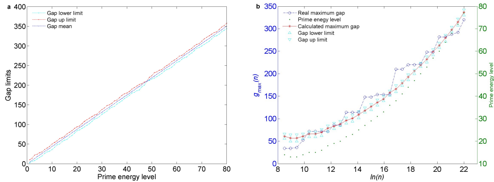
Fig. 5. Prediction on the maximum gaps changing with given prime numbers possessing different energy levels
