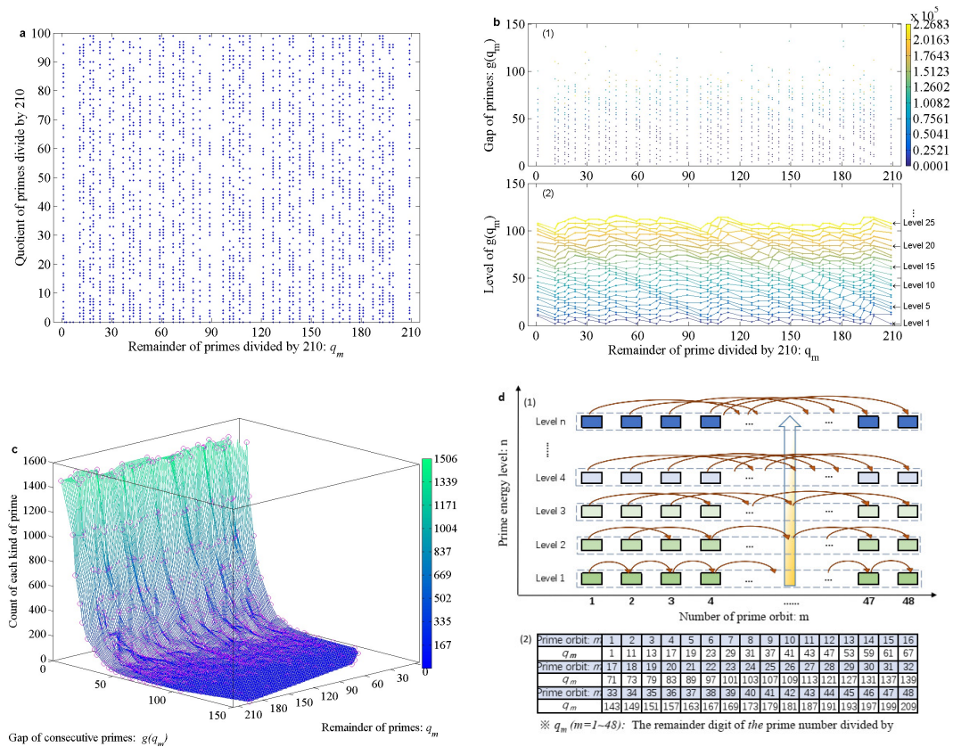
Fig. 1. Hierarchical progression phenomenon of prime gaps
