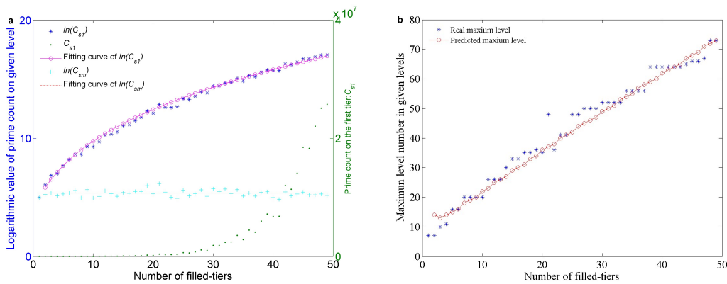
Fig. 4. Relationship between the maximum energy level and the filled tiers. a, The correlation curve of the filled tiers and the natural logarithm of count on prime numbers at a given level. b, The relationship between maximum energy level and the number of filled-tiers.
