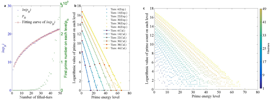
Fig. 3. Diagram of the maximum energy level and the filled tiers
