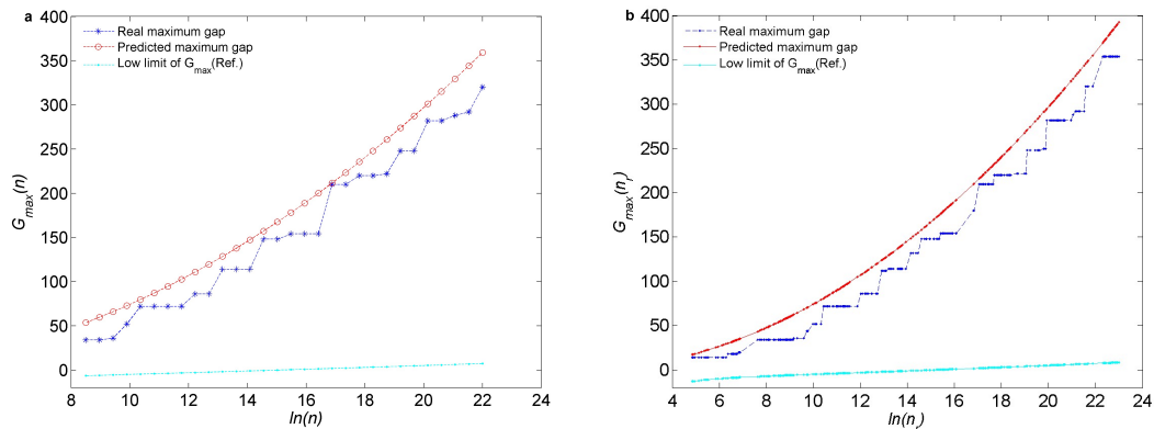
Fig. 6. Prediction on the maximum gaps between consecutive primes below a given number
