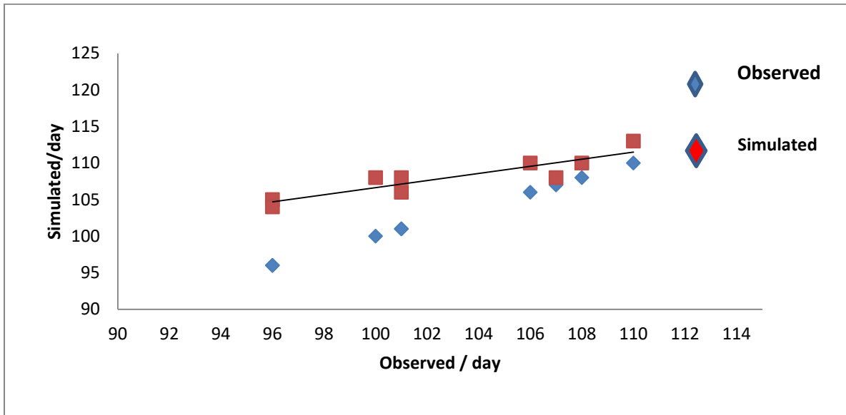
Fig. 2. Relationship between simulated and observed maturity (day) of wheat cultivars
