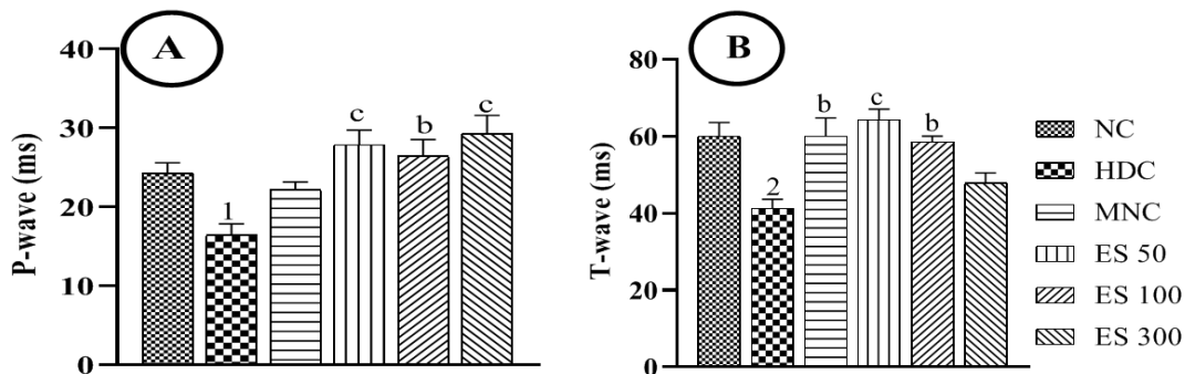
Fig. 3. Effects of E. senegalensis extract on the duration of atrial depolarisation (A) and ventricular repolarisation (B)
