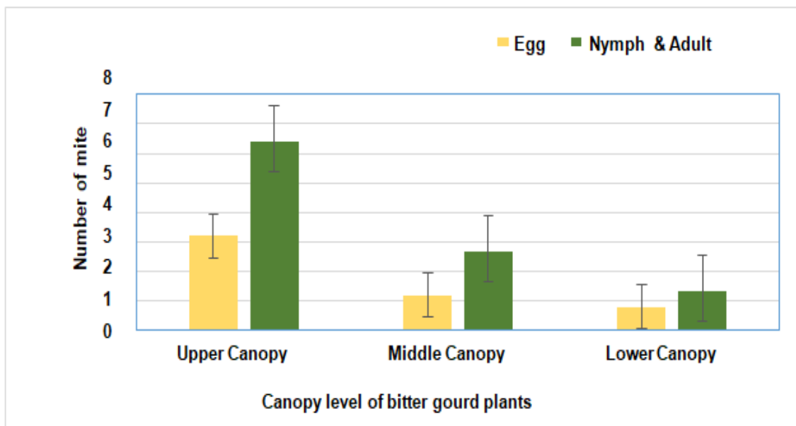
Fig. 1. Population of Tetranychus urticae Koch found in different canopy level of bitter gourd
