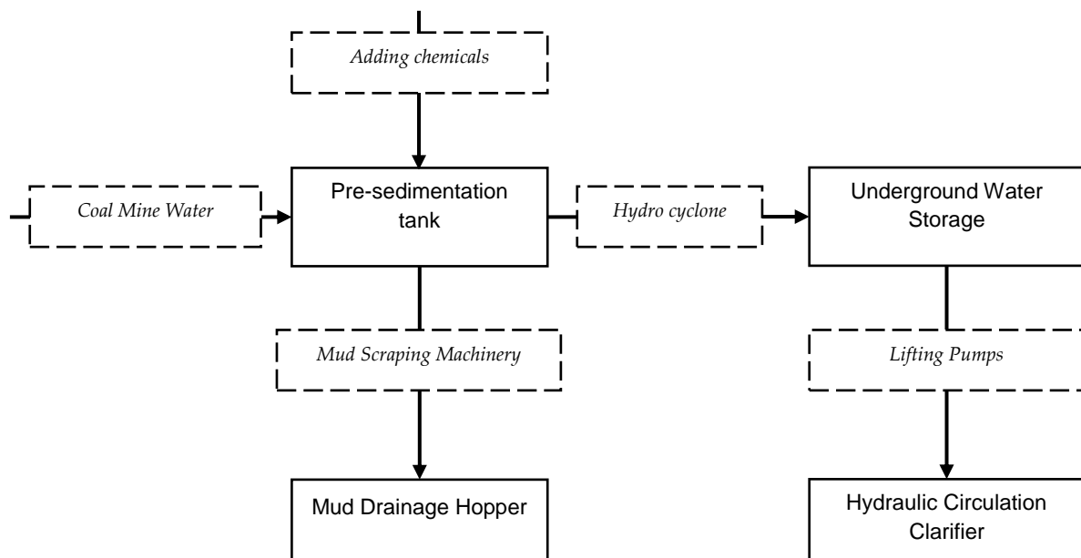
Fig. 2. Flow chart of coal mine water decontamination process
