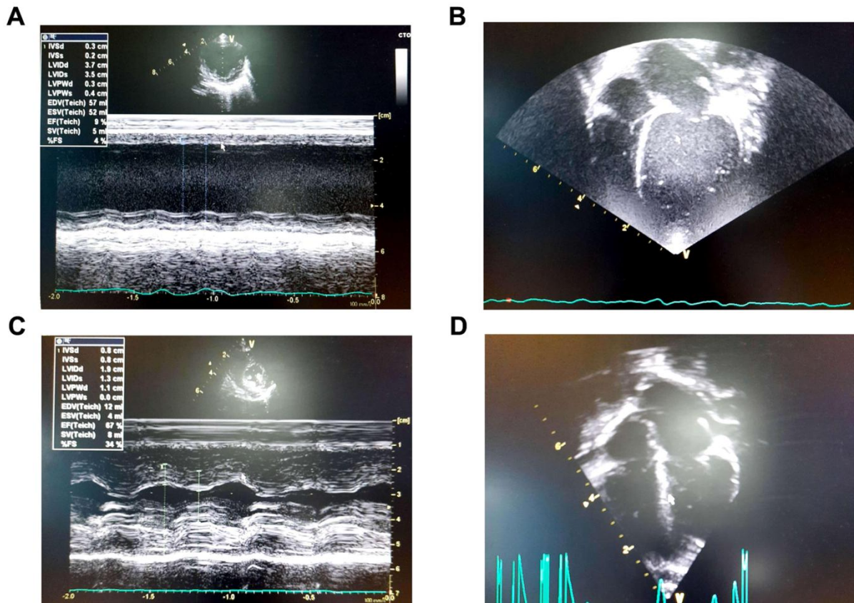
Fig. 1. Echocardiography finding in case 1. (A and C) M Mood (A) showed sever depressed Left Ventricle (LV) function with fractional shortening FS 4% and ejection fraction EF 9% on admission and (C) showed normal LV function with FS 34% and EF 67% on discharge. (B and D) Apical four chambers view (B) showed dilated Left Atrium (LA) and LV on admission and (D) showed balanced ventricles and resolved dilatation of LA and LV on discharge
