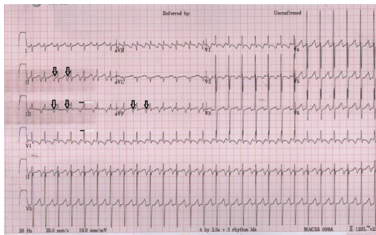
Fig. 3. 12 lead electrocardiography ECG in case 4, ECG demonstrate Permanent Junctional Reciprocating Tachycardia (PJRT) features, arrows showed inverted P wave in inferior leaders 11, 111, AVF and positive P wave in AVR , with longer RP interval (white horizontal lines) compare to PR interval ( black horizontal lines ) and narrow QRS complexes with 1:1 AV ratio (no dissociation)
