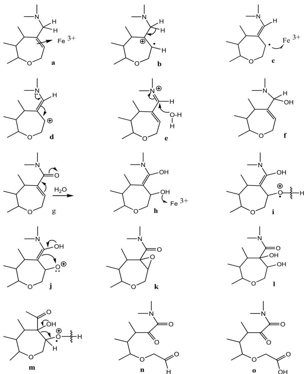
Fig. 2. Reaction route of the successive oxidations of strychnine in Davy test
