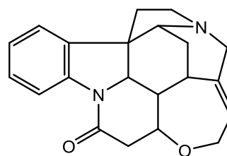
Fig. 1. Structure of strychnine
