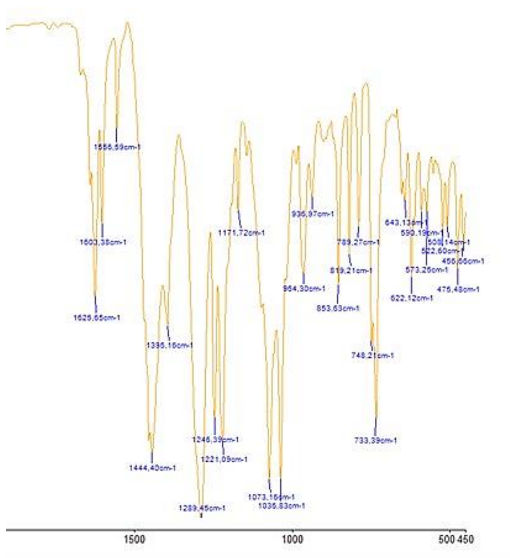
Fig. 1. Spectrum IR of complex [Cu_2(\mu-L)_2La(NO_3)_2]_2 \cdot La(NO_3)_4
