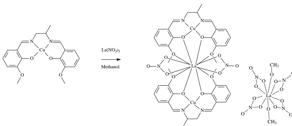
Scheme 5. Reaction scheme for the synthesis of the copper (II)/lanthanum (III) complex
