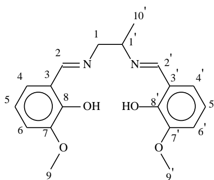
Scheme 3. Numbering of carbon atoms
