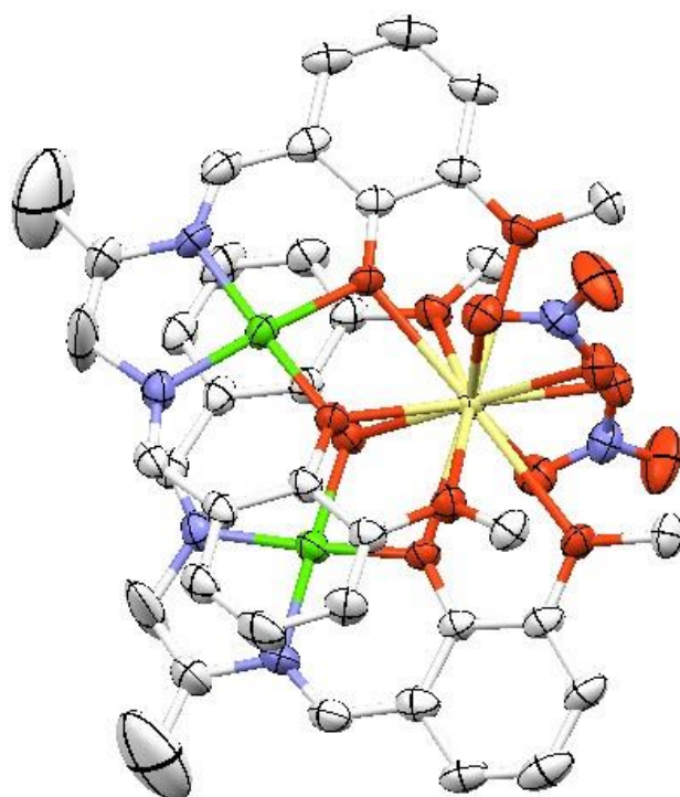
Fig. 4. ORTEP diagram of complex 2
