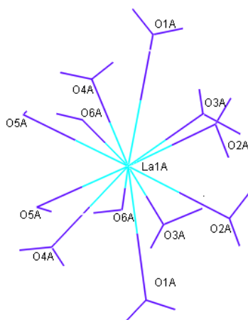
Fig. 7. Coordination scheme of La(III)
