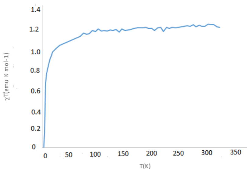
Fig. 2. \chi T = f(T) of complex [\text{Cu}_2(\mu\text{-L})_2\text{La}(\text{NO}_3)_2]_2\text{La}(\text{NO}_3)_4
