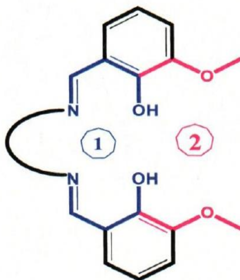
Scheme 1. Representation of the structure of a bicompartamental Schiff base
