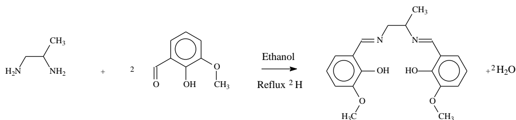
Scheme 2. Ligand synthesis reaction scheme
