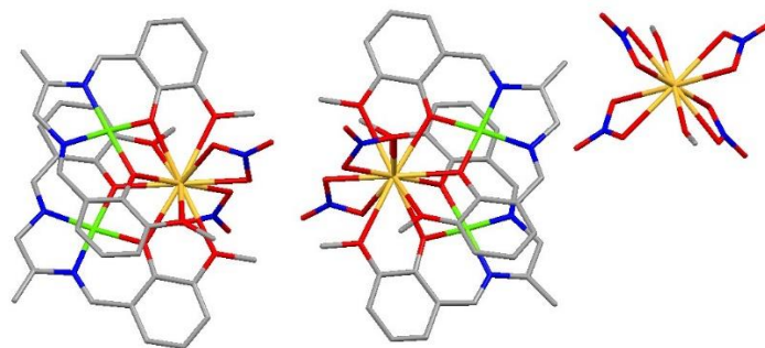
Fig. 6. Complete structure of complex 2 by capped sticks
