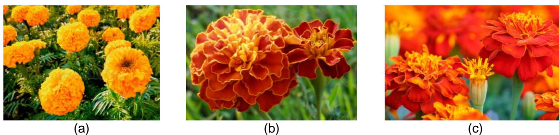
Fig. 1. (a) Tagetes erecta , (b) Tagetes patula , (c) Tagetes minuta
