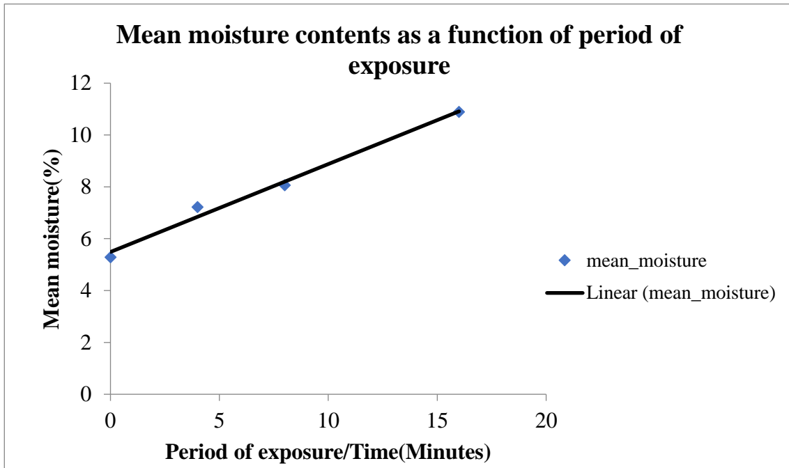
Fig. 2. Mean moisture contents versus period of exposure (soaking) in lime
