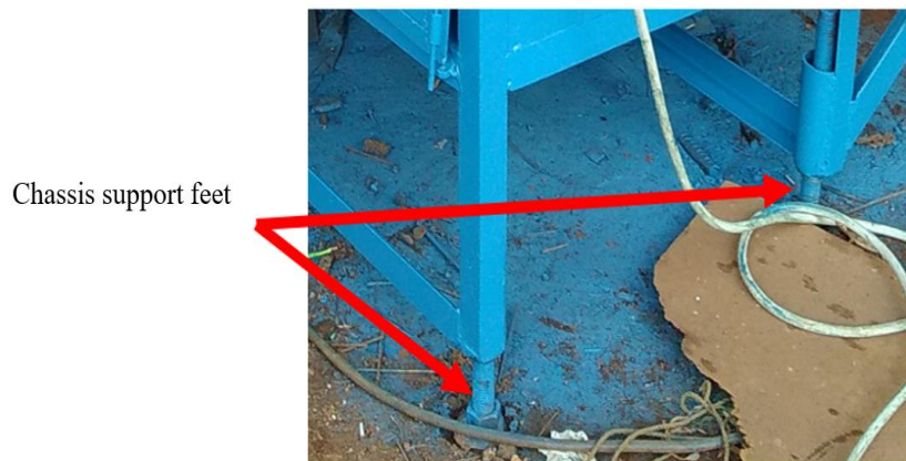
Fig. 10. Device for adjusting the angle of inclination of the roller taken at the end of manufacture
