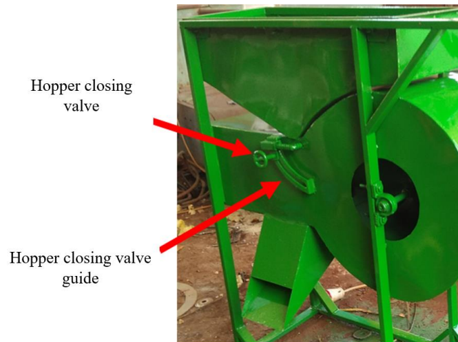
Fig. 5. Adjusting devices of the motorized winnower
