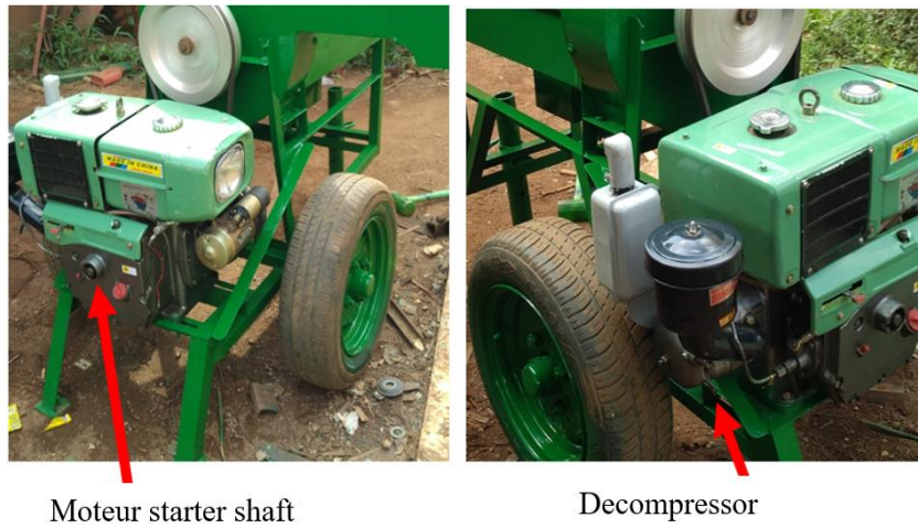
Fig. 3. Sheller motorization system
