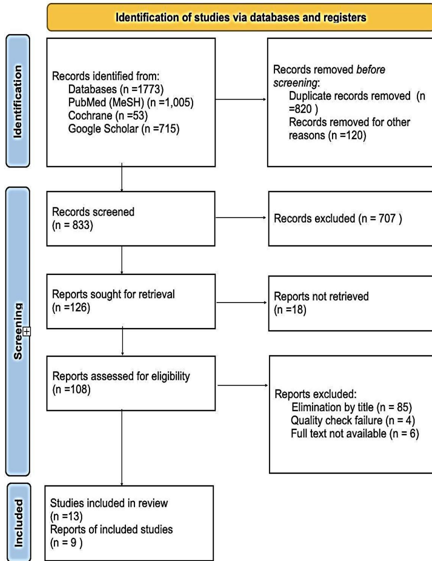
Fig. 1. PRISMA flowchart showing the process of article selection PRISMA: Preferred Reporting Items for Systematic Review and Meta-Analysis
