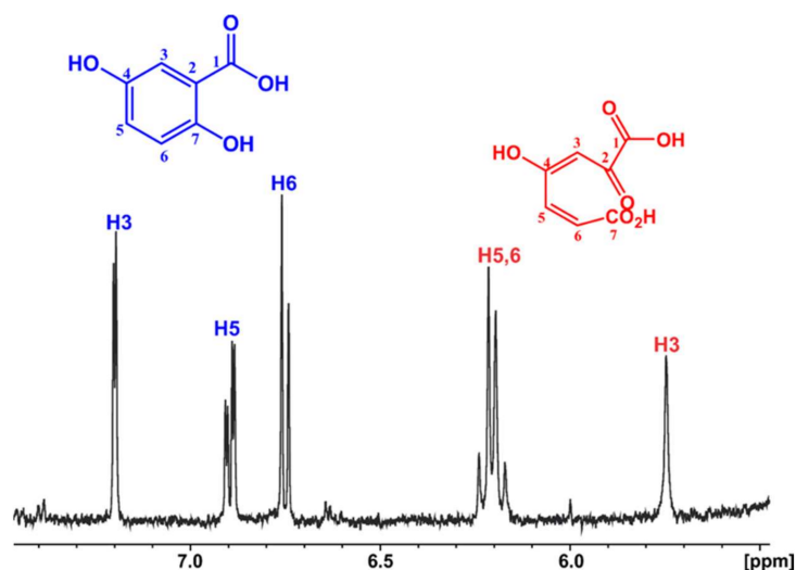
Figure 6. ^1\text{H} NMR spectrum of the gentisate (blue) biotransformation product, maleylpyruvate (red) in 50 mM Tris buffer 90% \text{H}_2\text{O} and 10% \text{D}_2\text{O} . (number of scans = 64, acquisition time = 4 s, relaxation delay = 1.5 s, total experimental time = 6 min 22 s).
