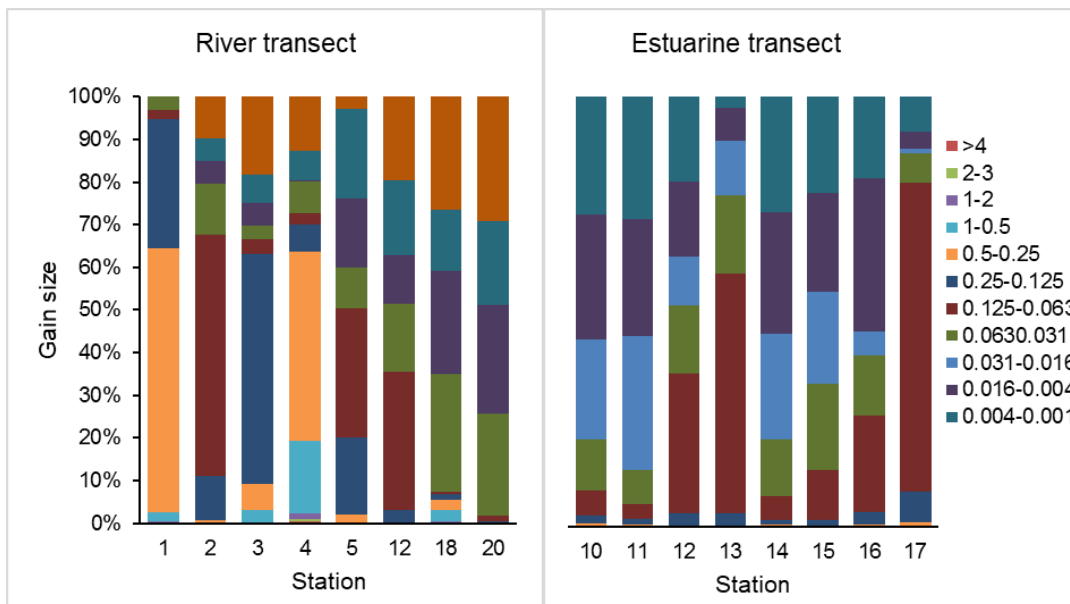
Fig. 3. Grain size of sediment in the river (left) and estuarine (right) transects
