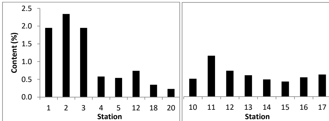
Fig. 2. Chlorophyll-a concentration in the river (left) and estuarine (right) transects
